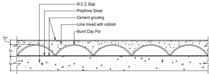
SECTION OF R.C.C. ROOF WITH BPRI
