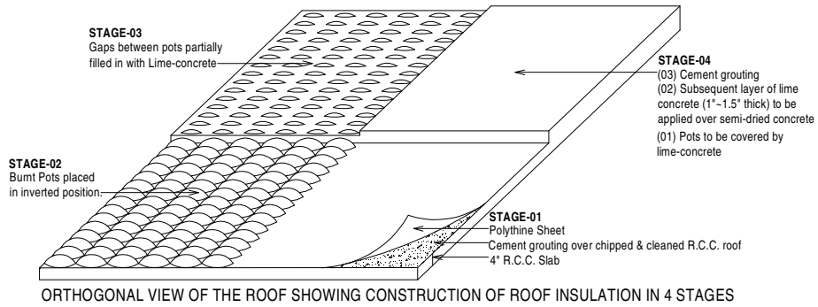
ORTHOGONAL VIEW OF THE ROOF SHOWING CONSTRUCTION OF ROOF INSULATION IN 4 STAGES
