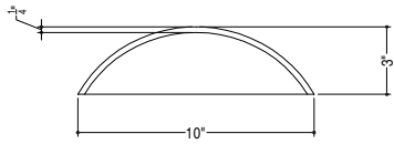
SECTION OF BURNT CLAY POT USED IN BPRI
