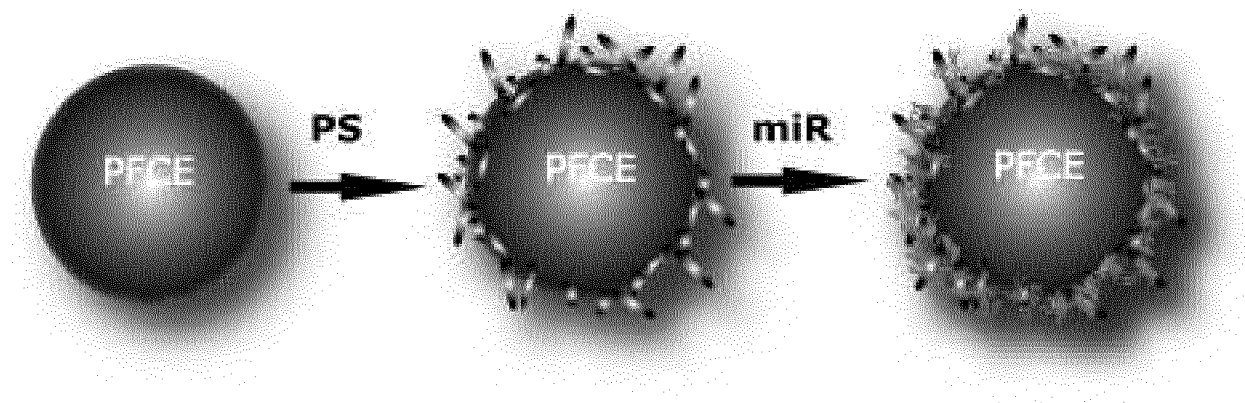
Fig 1. Preparation of the nanoparticle: conjugation of pefluorocarbon (PFCE) with protamine sulphate (PS) and the micro RNA therapeutic agent (miR).
